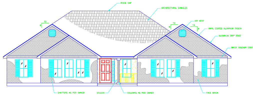
FRONT ELEVATION - ALT SCALE: 1/4" = 1'-0"
